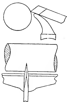
FIG. 310. USING TOE OF SKEW IN MAKING PREPARATORY CUT.
